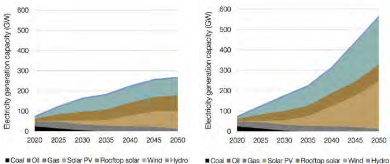
FIGURE 2.08: Renewable energy capacity in the ‘Coordinated action scenario’ (left) and ‘Coordinated action with exports sensitivity’ (right)
