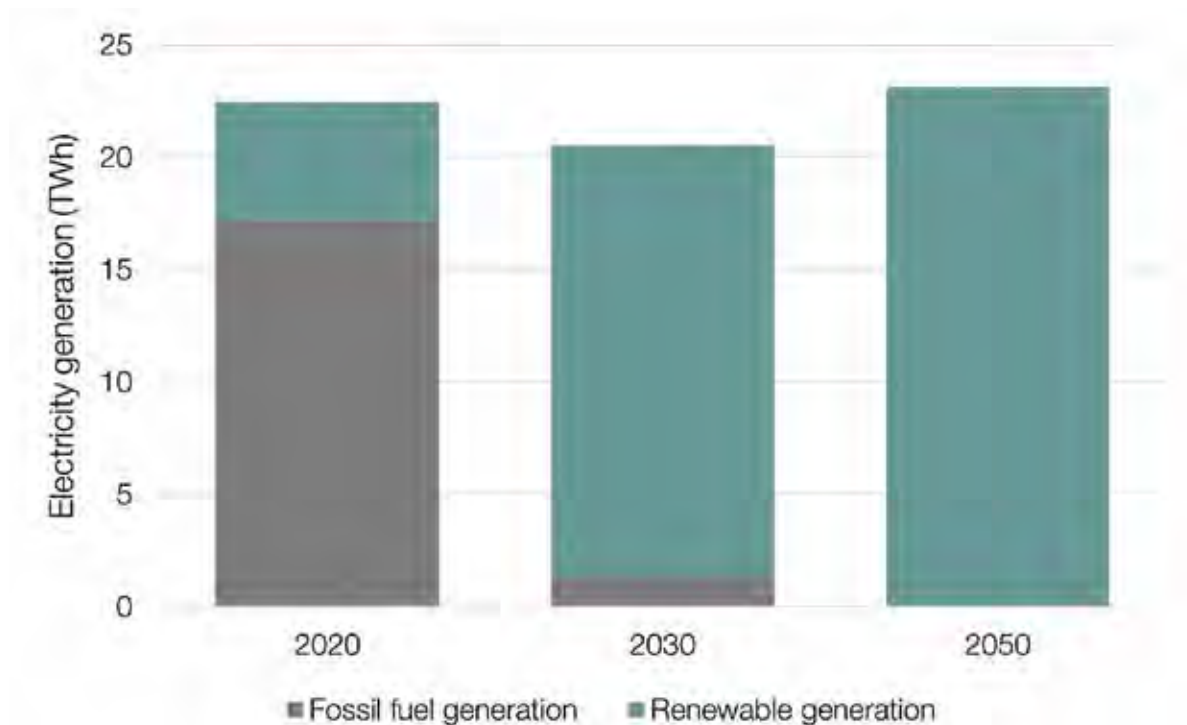
FIGURE 4.06: Electricity generated from fossil fuel and renewable sources for aluminium smelting
