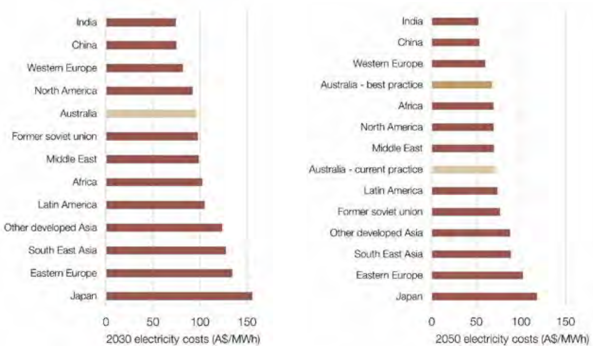
FIGURE 2.26: Global electricity costs in 2030 and 2050
