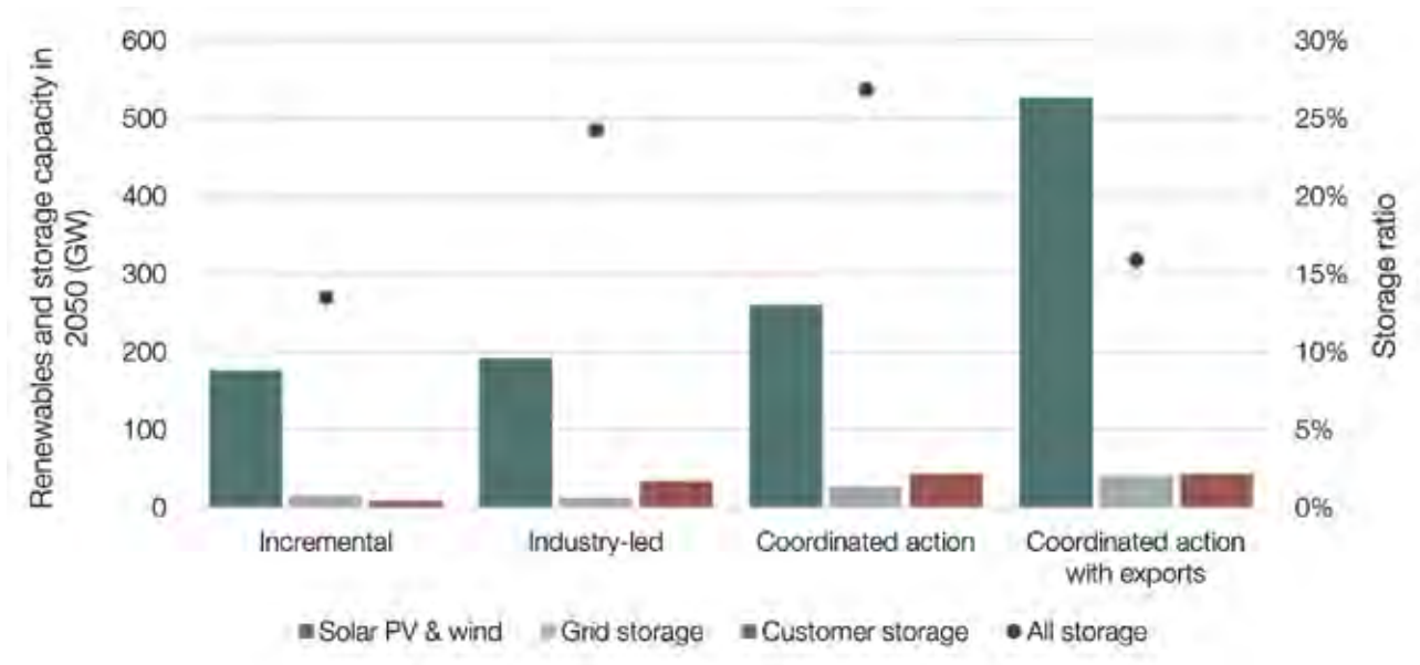
FIGURE 2.15: Storage capacity requirements in 2050 relative to renewable capacity
